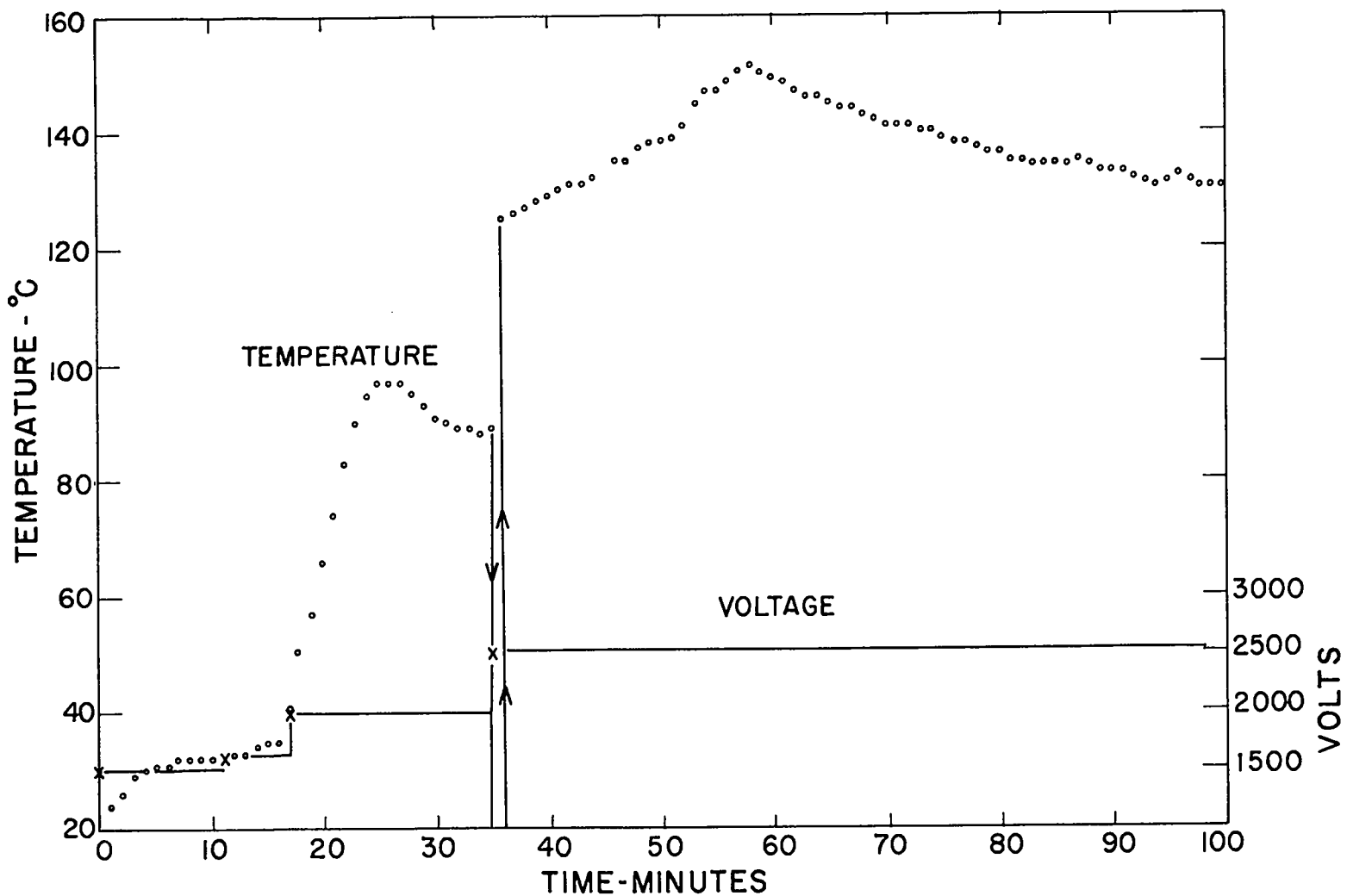
Fig. 6. Graph of temperature and voltage versus time for an alpha plutonium specimen in contact with the surface of the water-cooled cathode.
