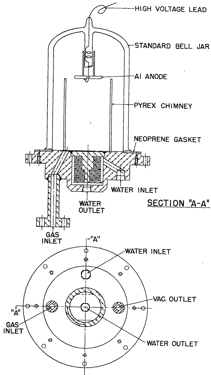
Fig. 1 Schematic diagram of glow discharge chamber.
