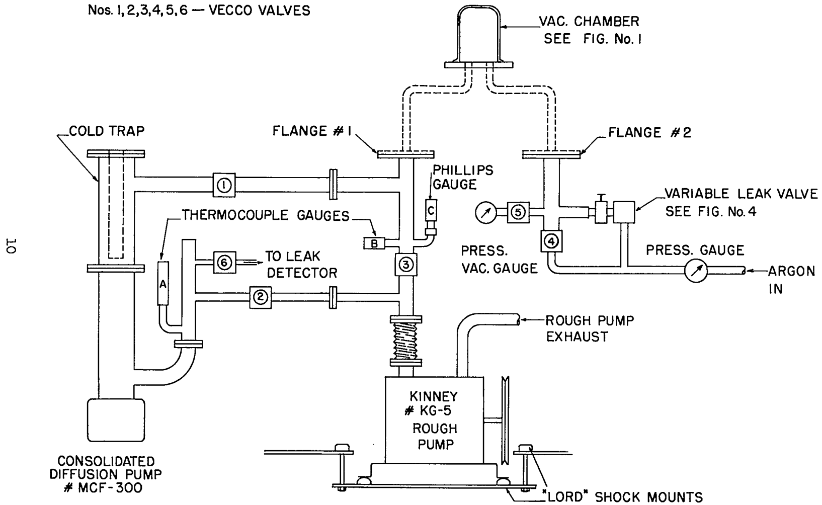
Fig. 2. Schematic diagram of vacuum system.
